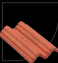
21 (204mm x 127mm) Rajwadi Round Channel Size : 8"x5" Per 100 Sq. Ft. 360 Nos 1 Sqm. = 39 Nos Weight Kg/Pc : 0.650
