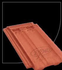
02 (407mm x 254mm) Double Groove Size : 16"x10" Per 100 Sq. Ft. 120 Nos 1 Sqm. = 13 Nos Weight Kg/Pc : 2.8
