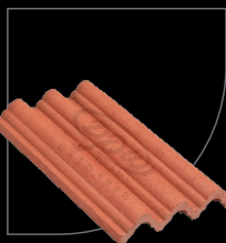
22 (204mm x 127mm) Triple Rajwadi Size : 8"x5" Per 100 Sq. Ft. 360 Nos 1 Sqm. = 39 Nos Weight Kg/Pc : 0.650
