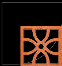
42 (204mm x 204mm) Four Petal Jaali Size : 8"x8" Per 100 Sq. Ft. 225 Nos 1 Sqm. = 25 Nos Weight Kg/Pc : 2.5
