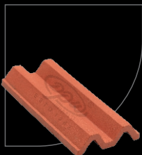
18 (204mm x 102mm) Double Channel Size : 8"x4" Per 100 Sq. Ft. 450 Nos 1 Sqm. = 49 Nos Weight Kg/Pc : 0.550
