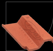
9 (178mm x 127mm) Mini Italian Tailor Size : 7"x5" Per 100 Sq. Ft. 625 Nos 1 Sqm. = 68 Nos Weight Kg/Pc : 0.500
